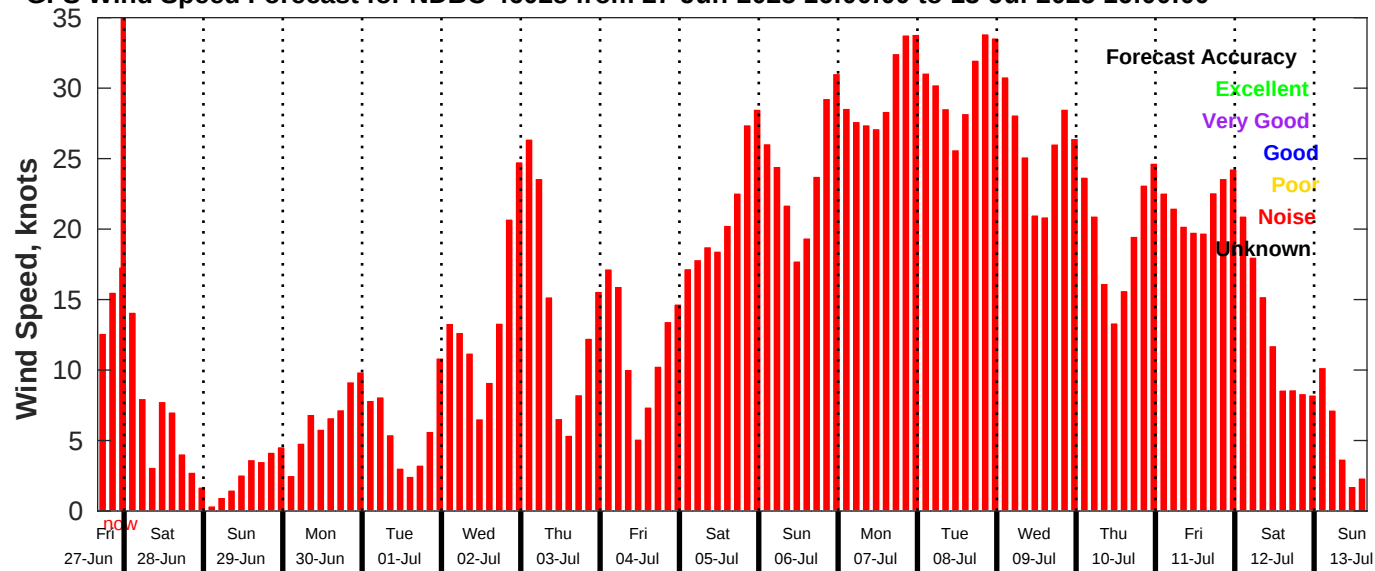
GFS Wind Speed Forecast for NDBC 46028 from 27-Jun-2025 16:00:00 to 13-Jul-2025 16:00:00
