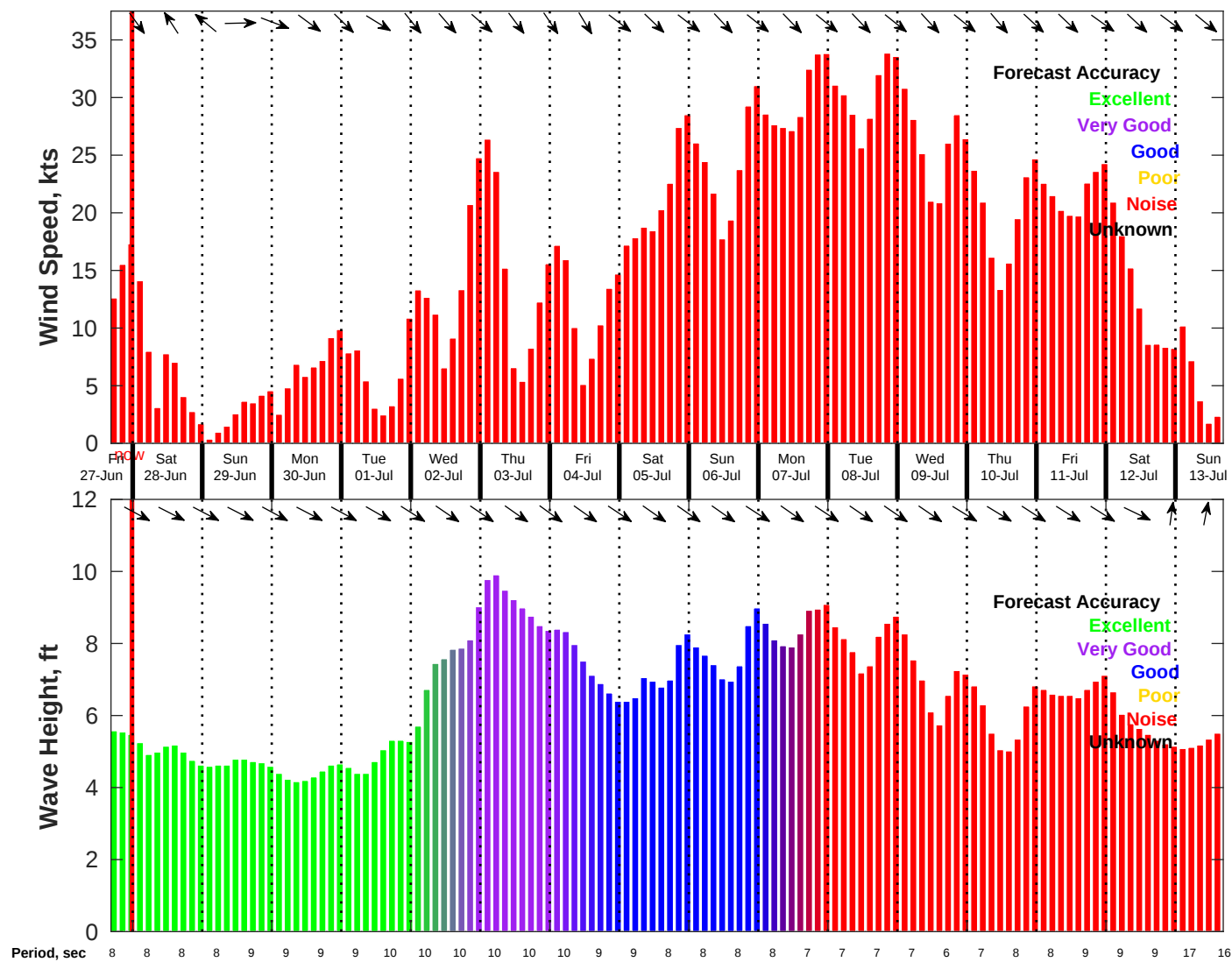
Wind & Wave Forecast for NDBC 46028 from 27-Jun-2025 16:00:00 to 13-Jul-2025 16:00:00
