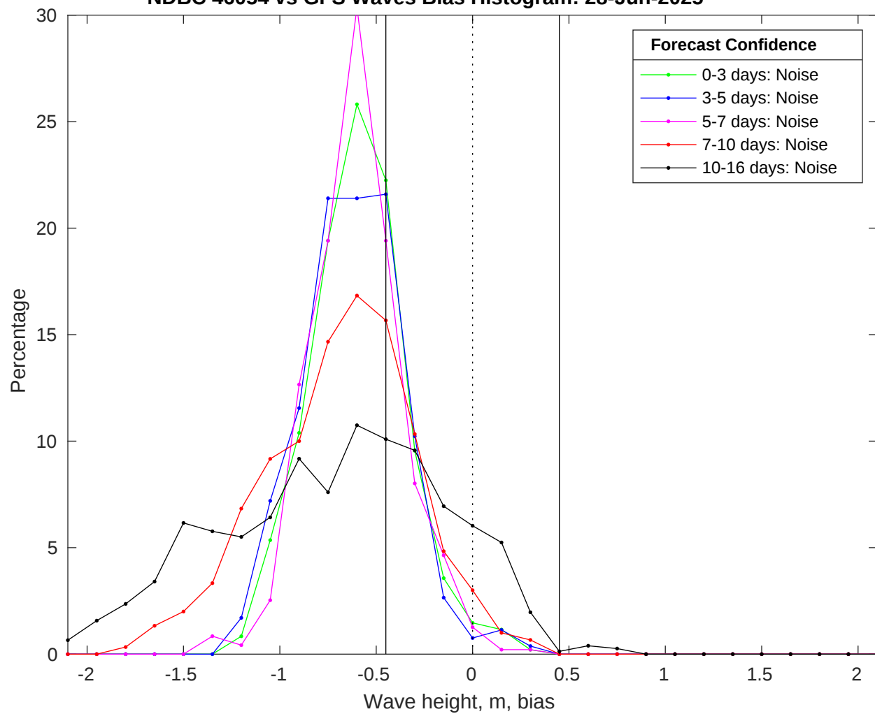
NDBC 46054 vs GFS Waves Bias Histogram: 28-Jun-2025
