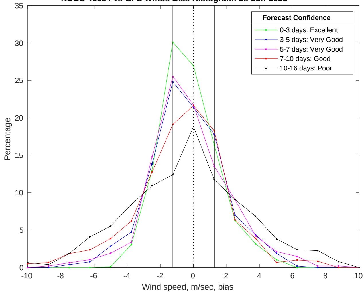
NDBC 46054 vs GFS Winds Bias Histogram: 28-Jun-2025
