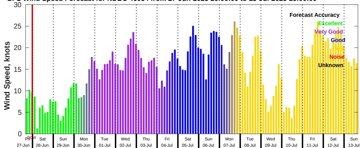
GFS Wind Speed Forecast for NDBC 46054 from 27-Jun-2025 16:00:00 to 13-Jul-2025 16:00:00
