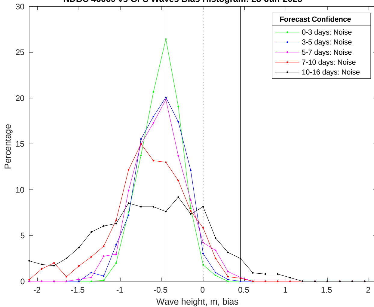
NDBC 46069 vs GFS Waves Bias Histogram: 28-Jun-2025
