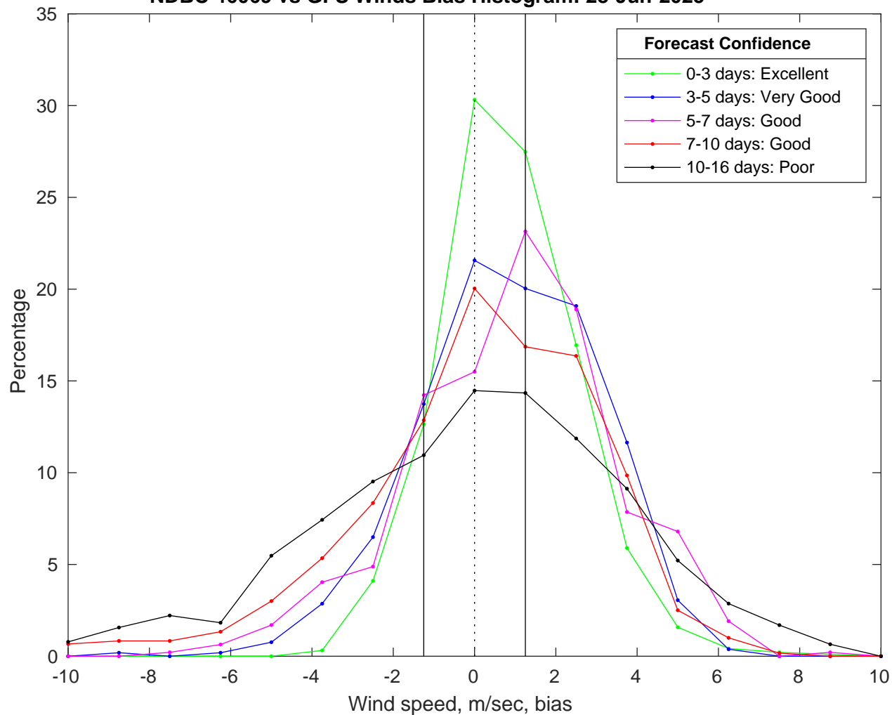
NDBC 46069 vs GFS Winds Bias Histogram: 28-Jun-2025
