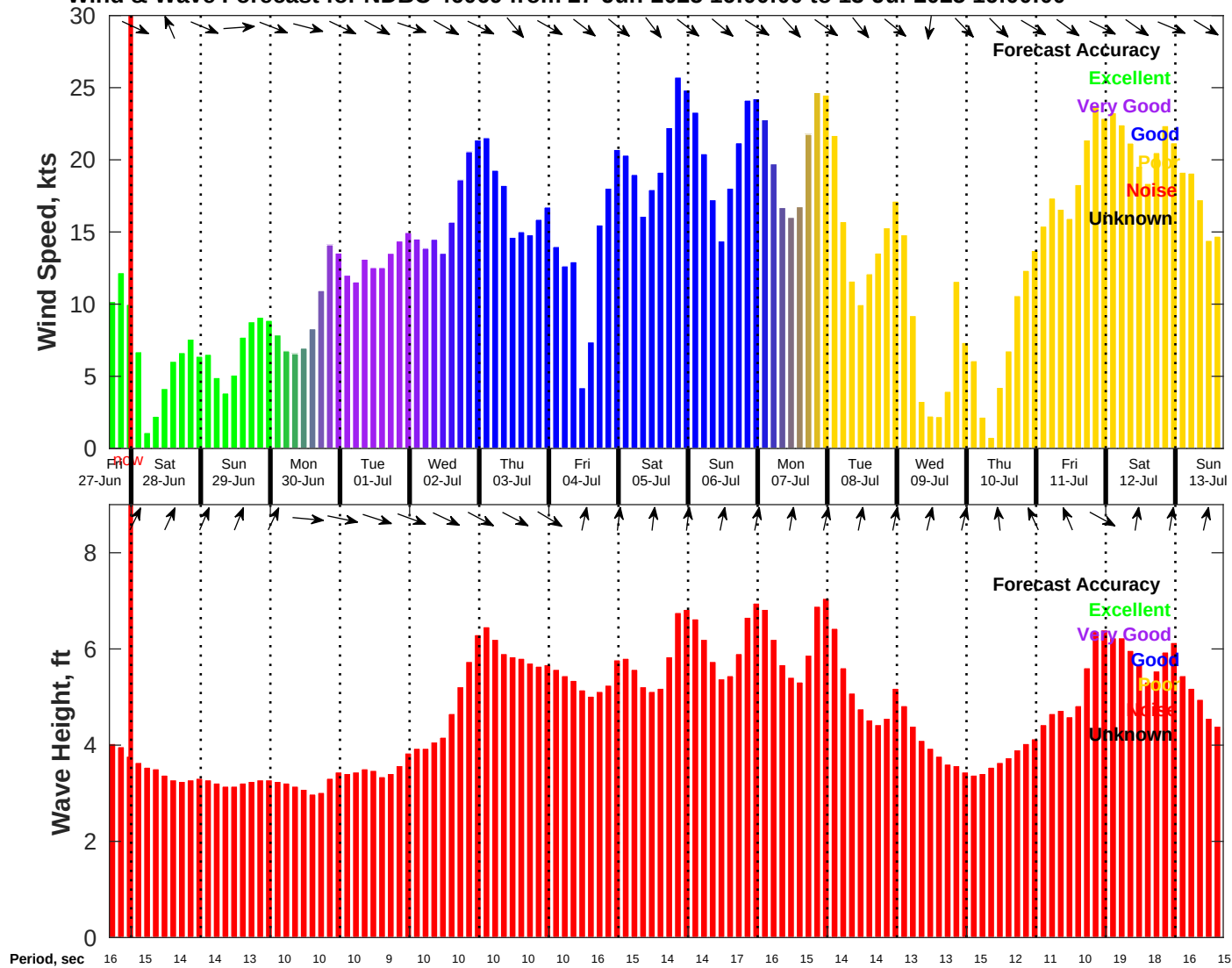
Wind & Wave Forecast for NDBC 46069 from 27-Jun-2025 16:00:00 to 13-Jul-2025 16:00:00
