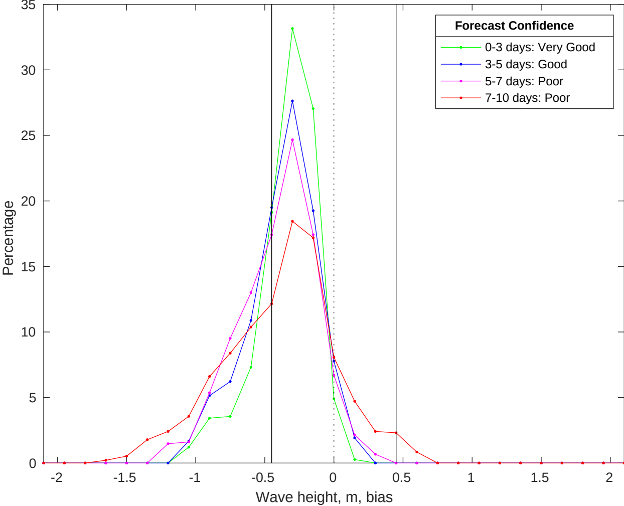
NDBC 51209 vs CMEMS Waves Bias Histogram: 28-Jun-2025
