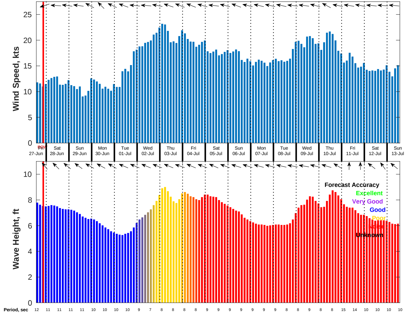
Wind & Wave Forecast for NDBC 51209 from 27-Jun-2025 13:00:00 to 13-Jul-2025 13:00:00
