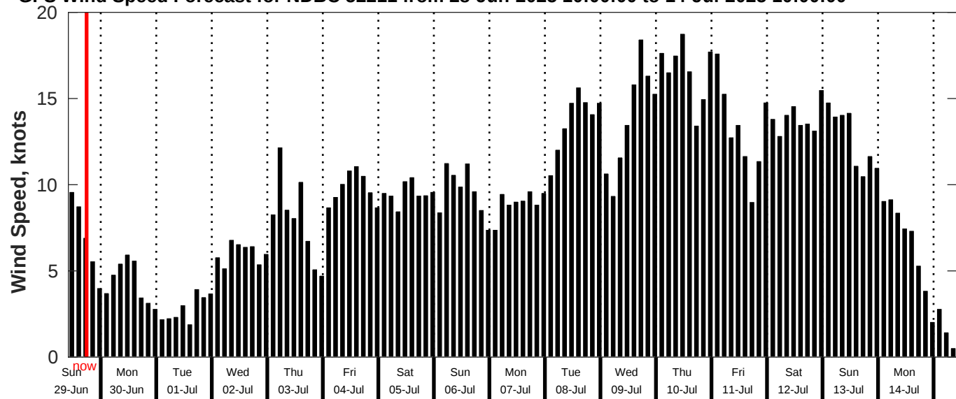
GFS Wind Speed Forecast for NDBC 52211 from 28-Jun-2025 10:00:00 to 14-Jul-2025 10:00:00
