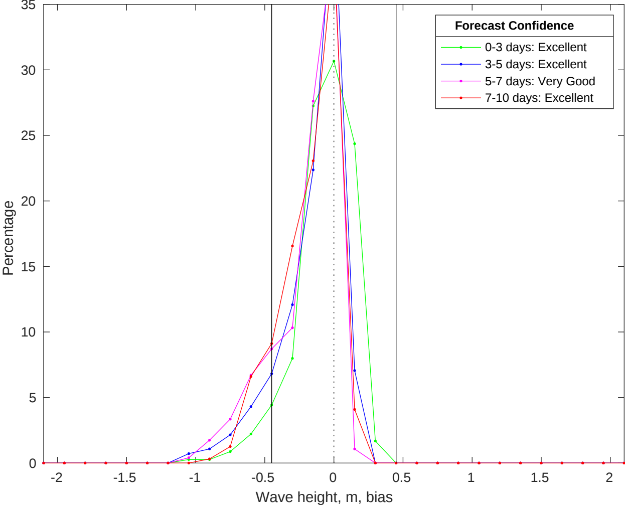
NDBC 52212 vs CMEMS Waves Bias Histogram: 28-Jun-2025
