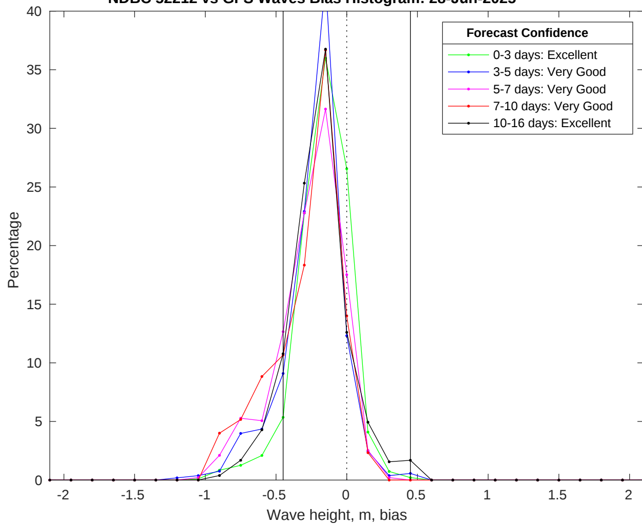
NDBC 52212 vs GFS Waves Bias Histogram: 28-Jun-2025
