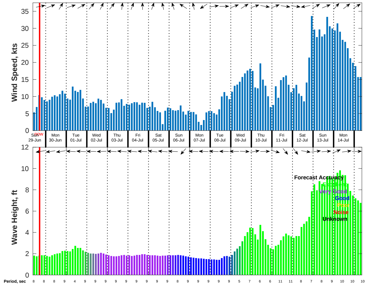
Wind & Wave Forecast for NDBC 52212 from 28-Jun-2025 09:00:00 to 14-Jul-2025 09:00:00
