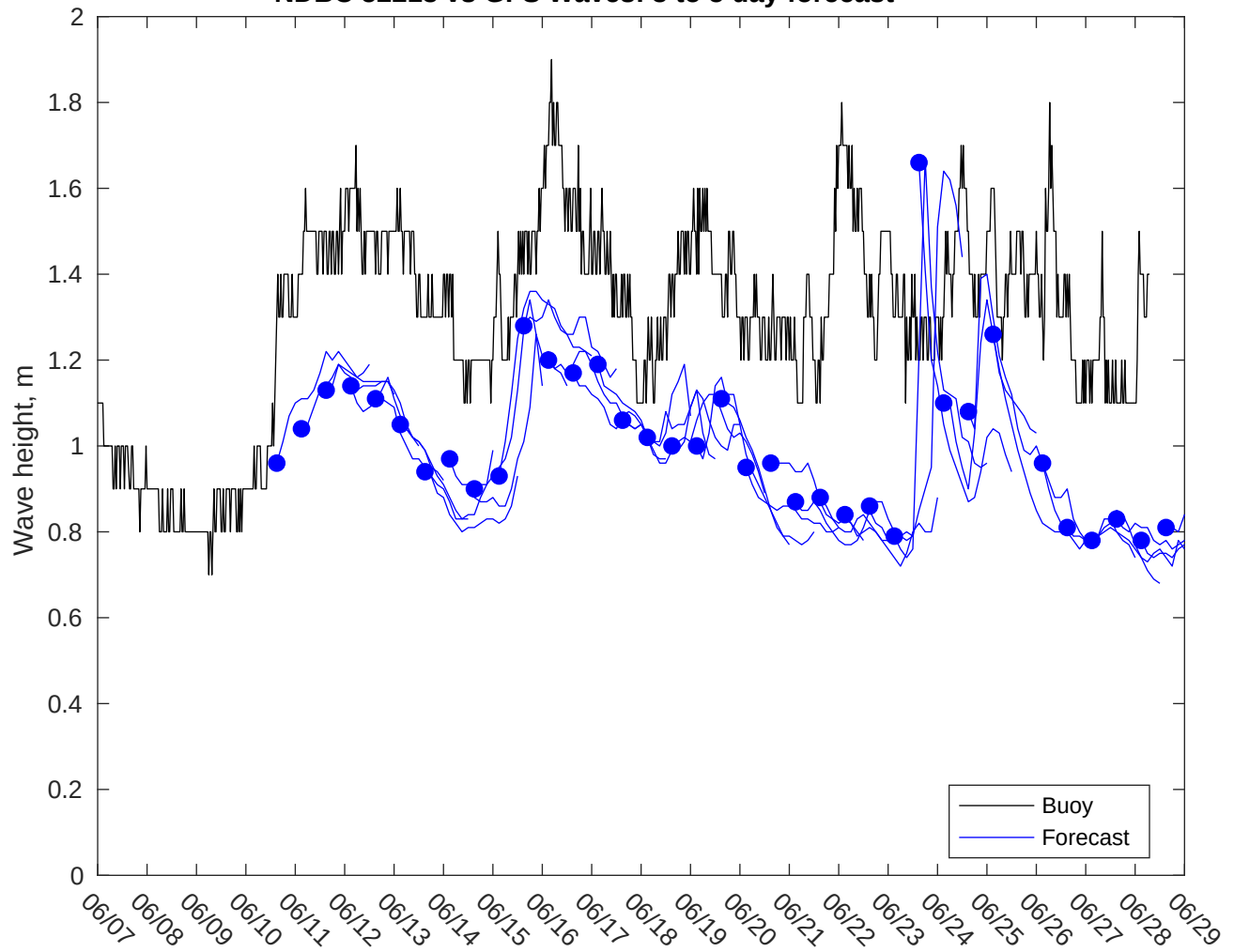
NDBC 52213 vs GFS Waves: 3 to 5 day forecast
