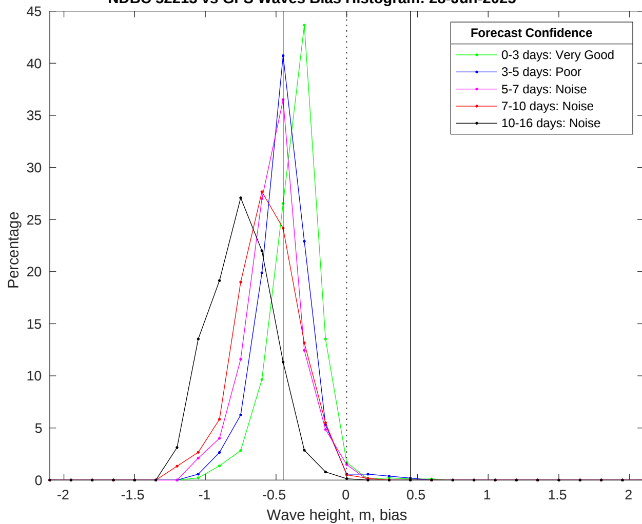
NDBC 52213 vs GFS Waves Bias Histogram: 28-Jun-2025
