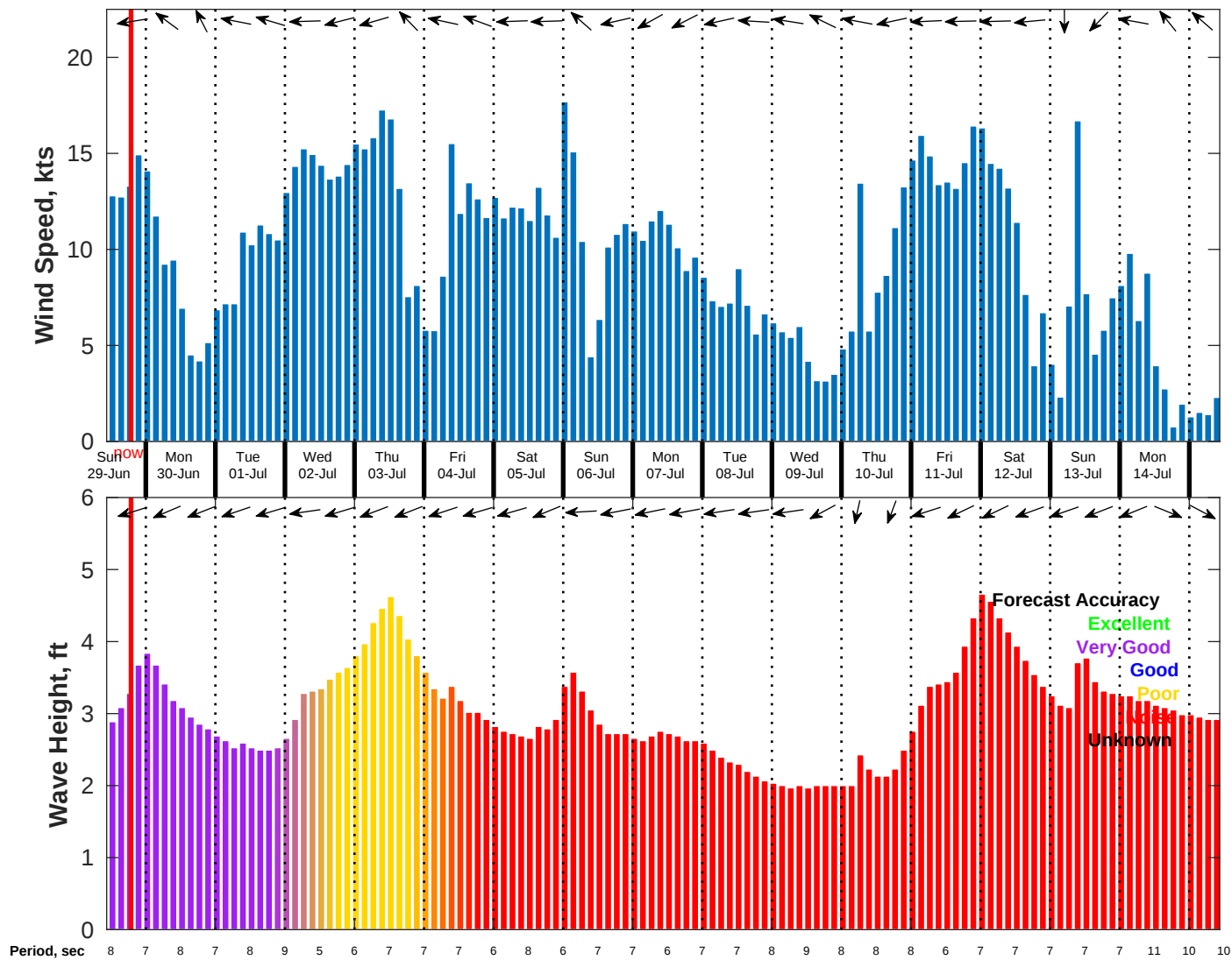
Wind & Wave Forecast for NDBC 52213 from 28-Jun-2025 11:00:00 to 14-Jul-2025 11:00:00
