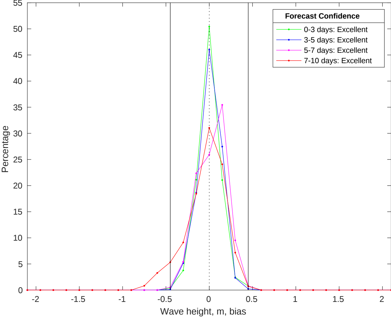
NDBC 41004 vs CMEMS Waves Bias Histogram: 29-Jun-2025
