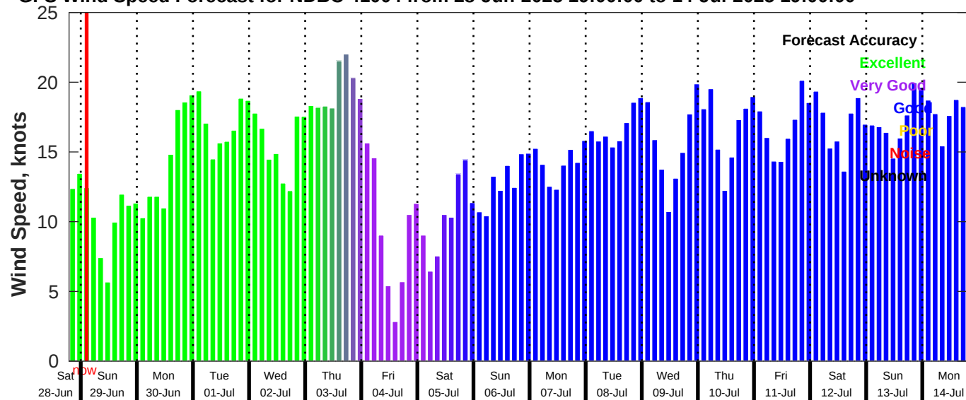
GFS Wind Speed Forecast for NDBC 41004 from 28-Jun-2025 19:00:00 to 14-Jul-2025 19:00:00
