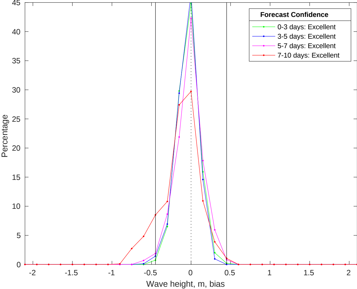
NDBC 41013 vs CMEMS Waves Bias Histogram: 29-Jun-2025
