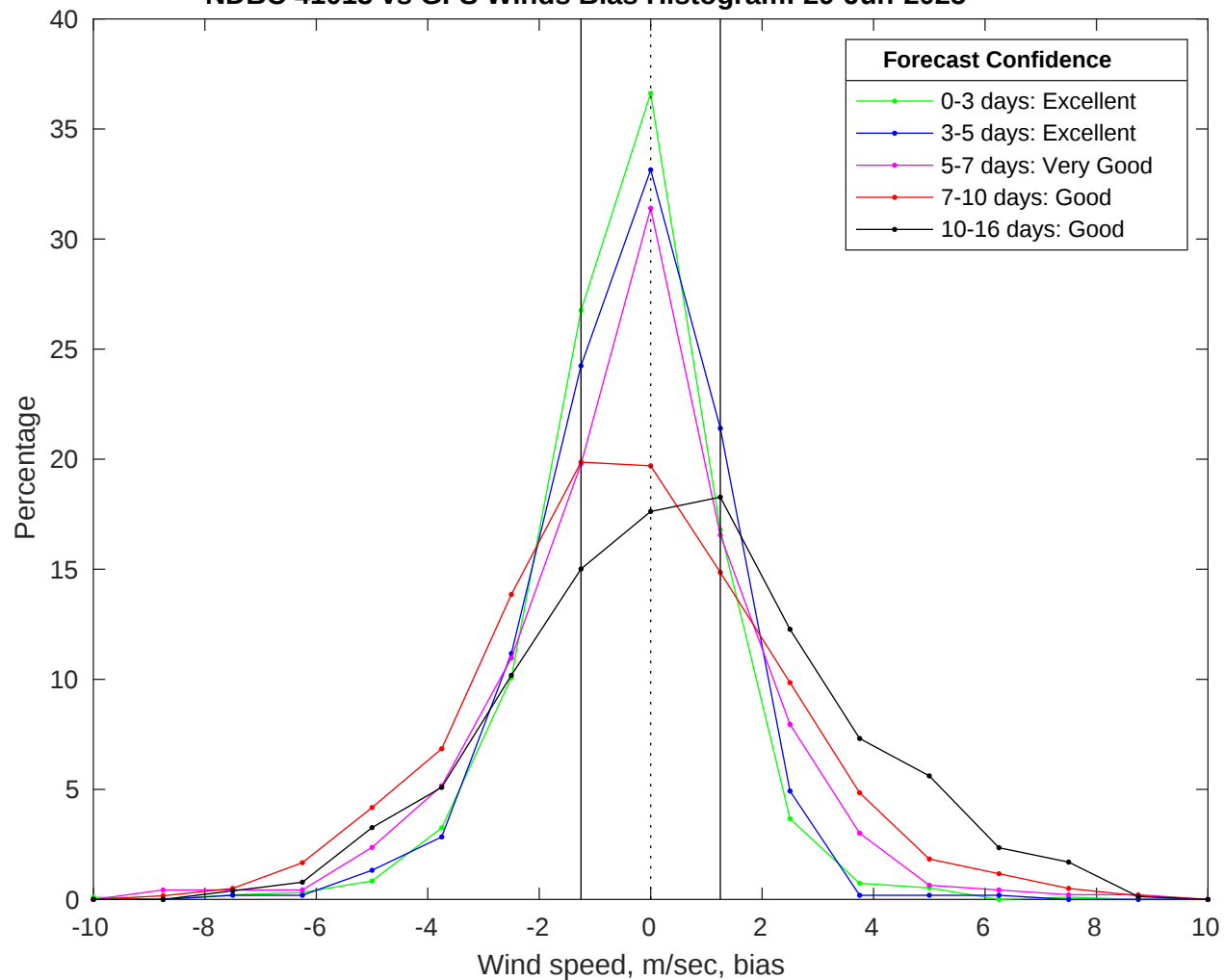
NDBC 41013 vs GFS Winds Bias Histogram: 29-Jun-2025
