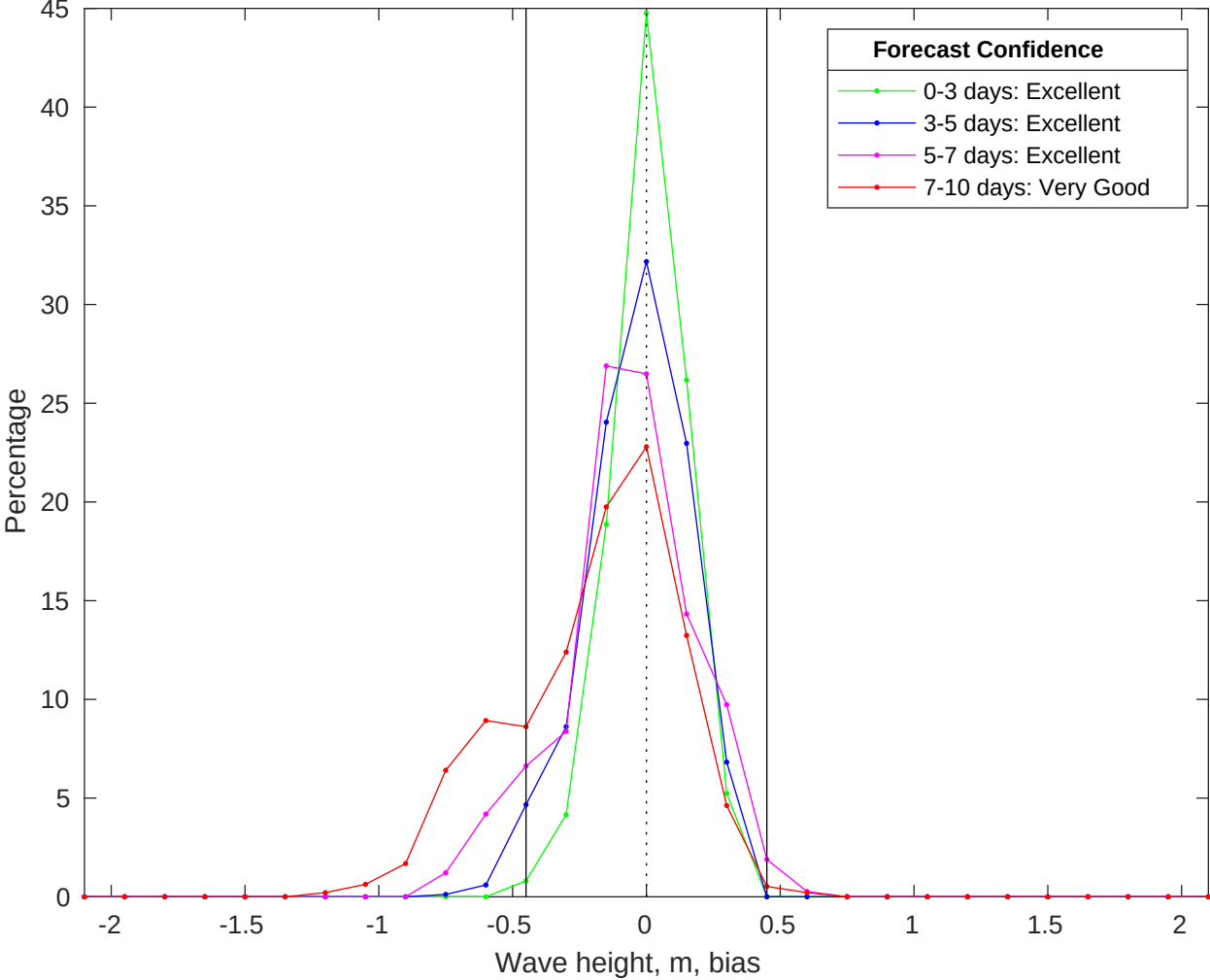
NDBC 41040 vs CMEMS Waves Bias Histogram: 29-Jun-2025
