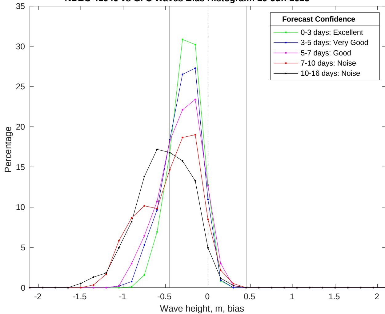
NDBC 41040 vs GFS Waves Bias Histogram: 29-Jun-2025
