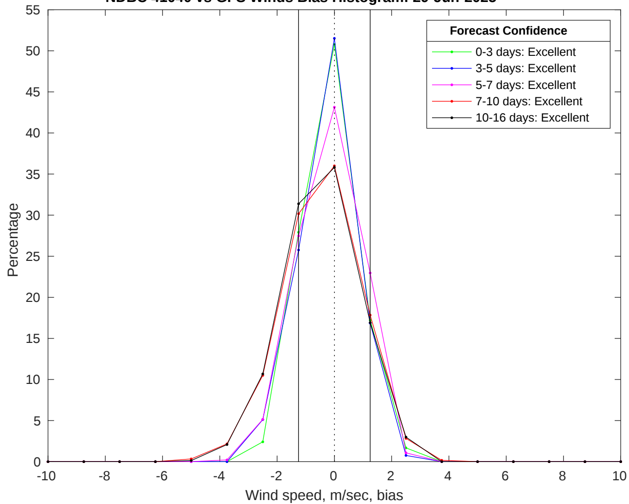
NDBC 41040 vs GFS Winds Bias Histogram: 29-Jun-2025
