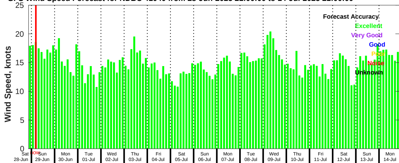
GFS Wind Speed Forecast for NDBC 41040 from 28-Jun-2025 21:00:00 to 14-Jul-2025 21:00:00
