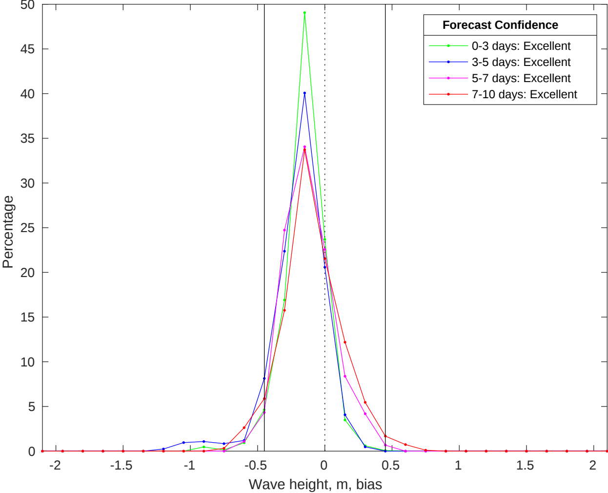
NDBC 42019 vs CMEMS Waves Bias Histogram: 29-Jun-2025
