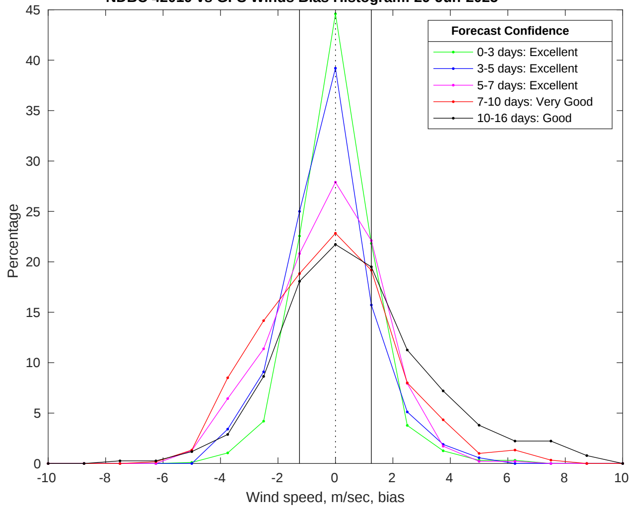
NDBC 42019 vs GFS Winds Bias Histogram: 29-Jun-2025
