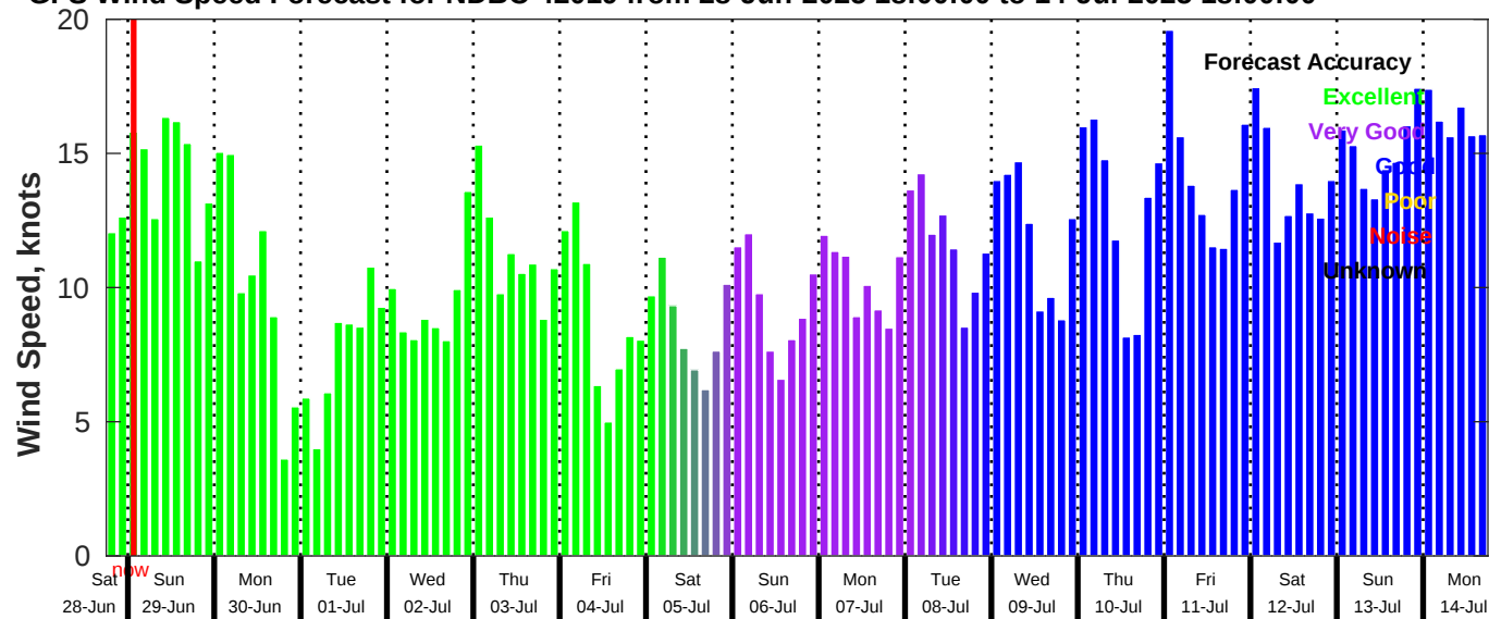
GFS Wind Speed Forecast for NDBC 42019 from 28-Jun-2025 18:00:00 to 14-Jul-2025 18:00:00
