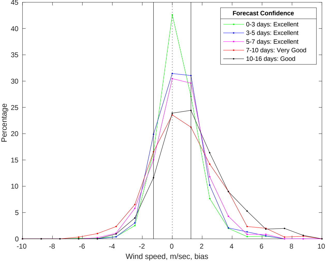
NDBC 42020 vs GFS Winds Bias Histogram: 29-Jun-2025
