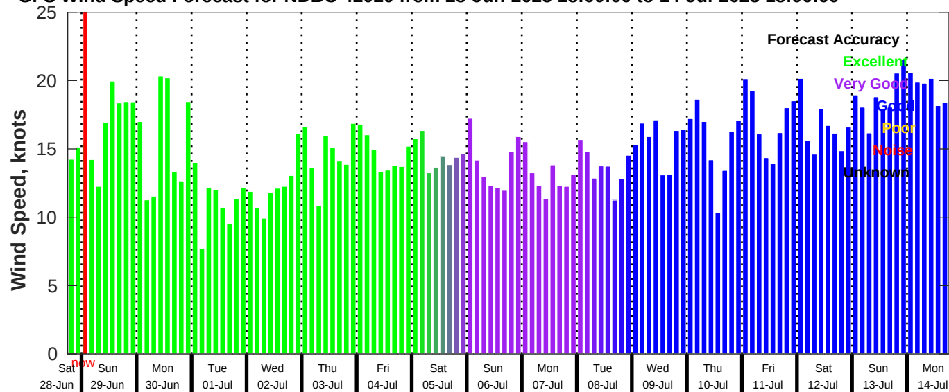
GFS Wind Speed Forecast for NDBC 42020 from 28-Jun-2025 18:00:00 to 14-Jul-2025 18:00:00
