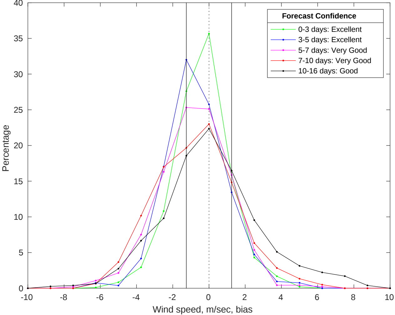
NDBC 42035 vs GFS Winds Bias Histogram: 29-Jun-2025
