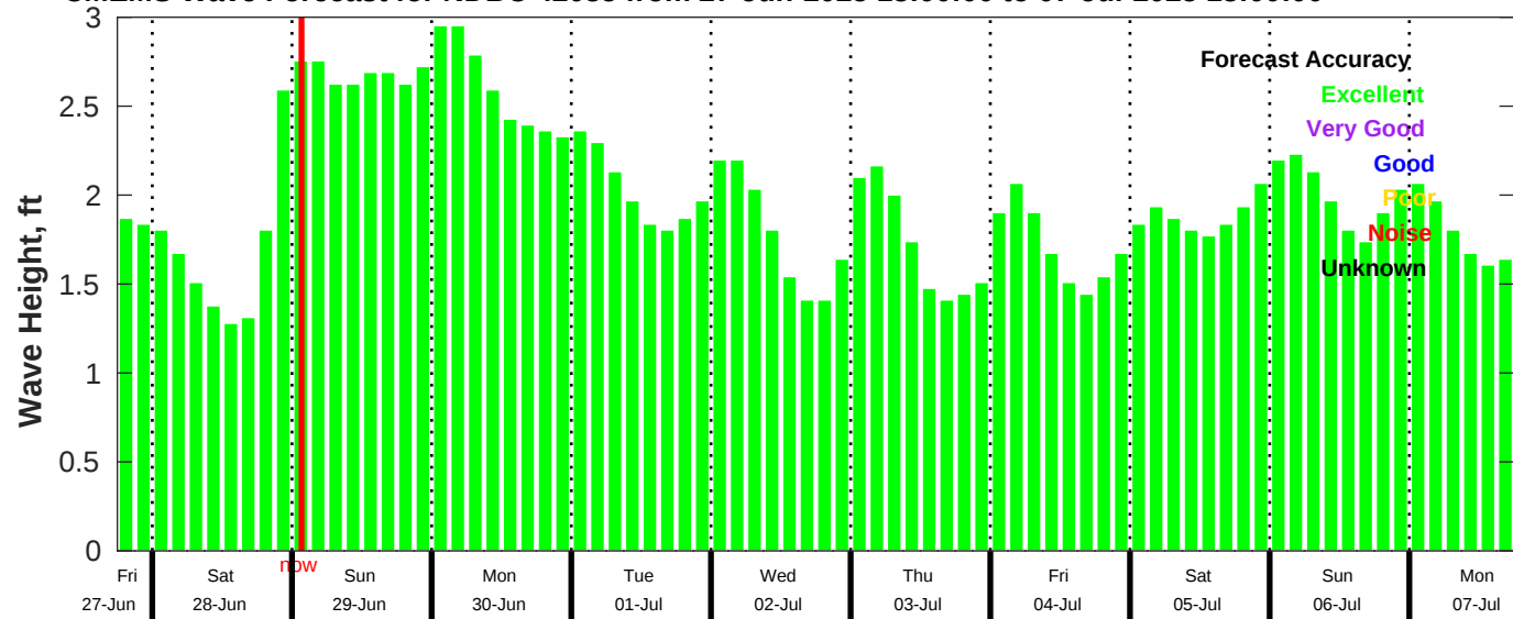
CMEMS Wave Forecast for NDBC 42035 from 27-Jun-2025 18:00:00 to 07-Jul-2025 18:00:00
