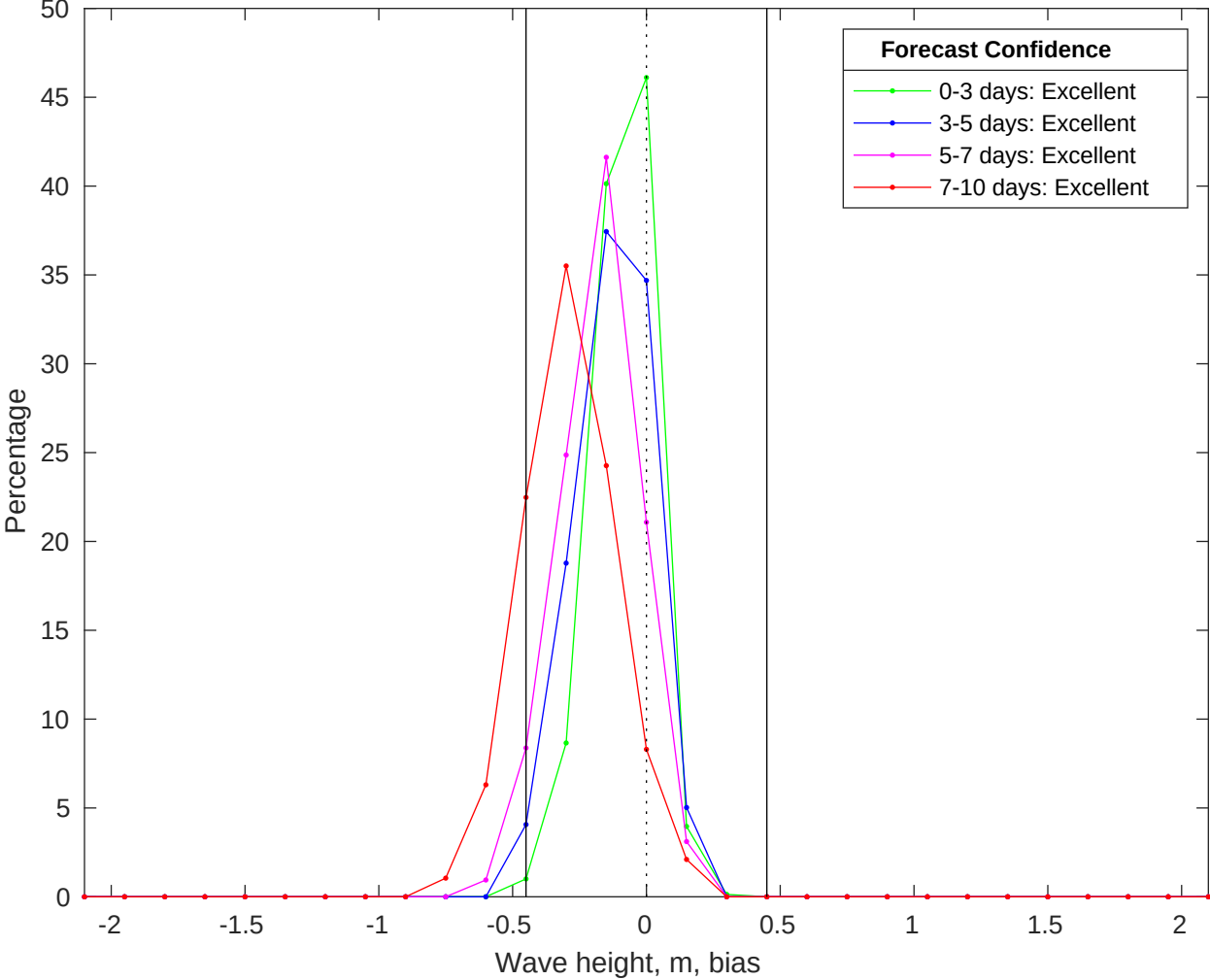
NDBC 42036 vs CMEMS Waves Bias Histogram: 29-Jun-2025
