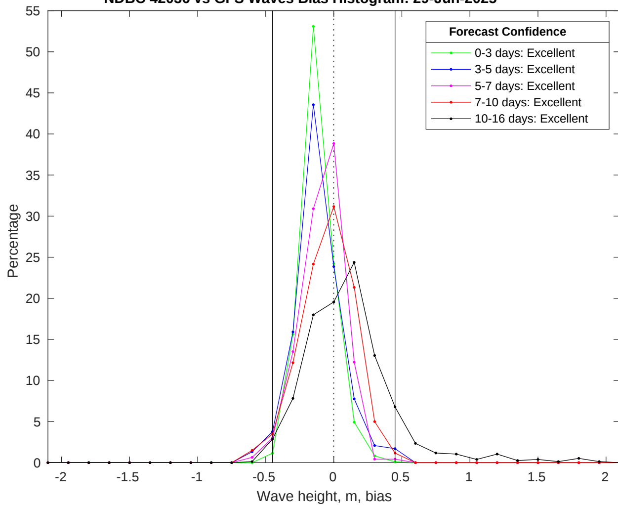
NDBC 42036 vs GFS Waves Bias Histogram: 29-Jun-2025
