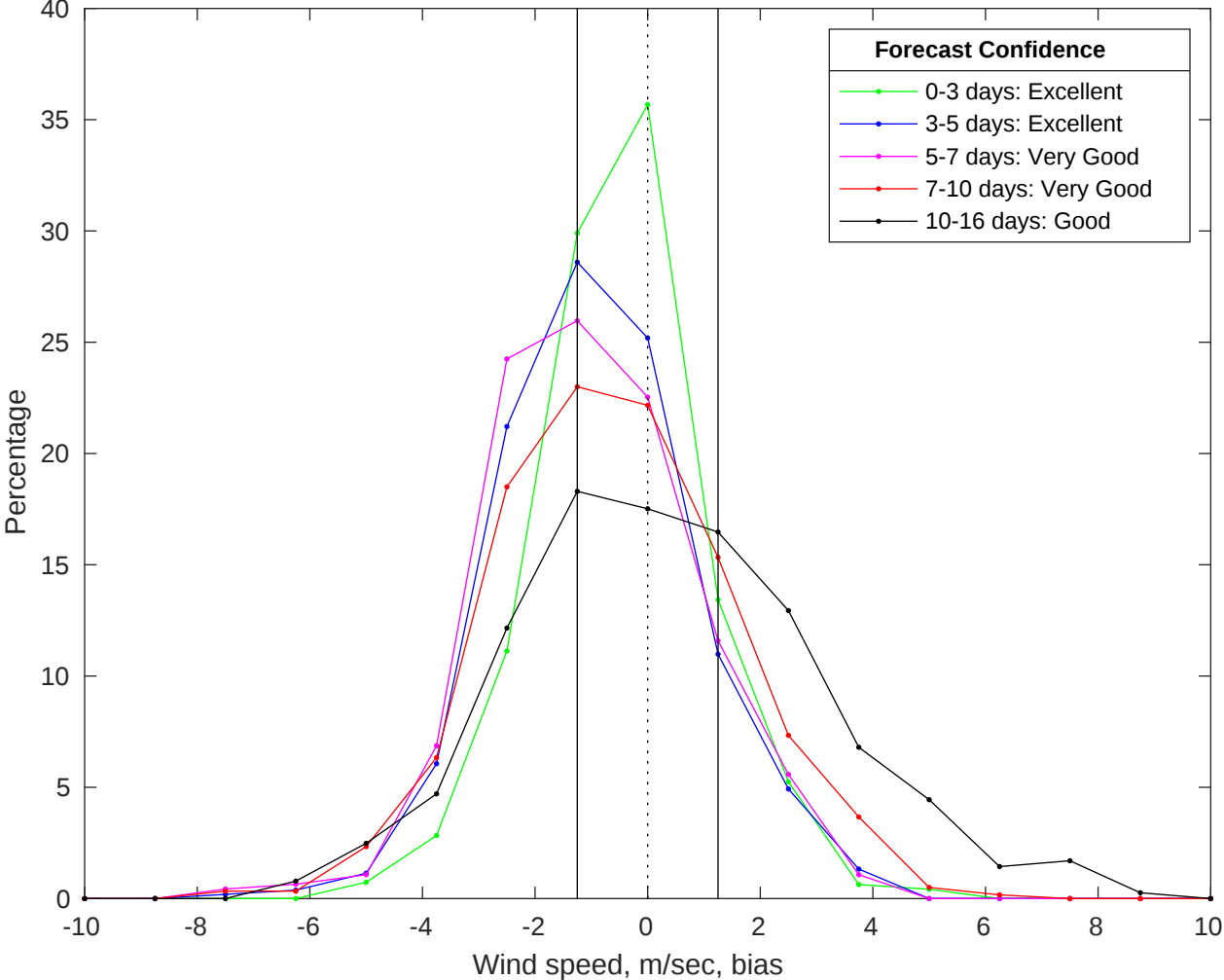
NDBC 42036 vs GFS Winds Bias Histogram: 29-Jun-2025
