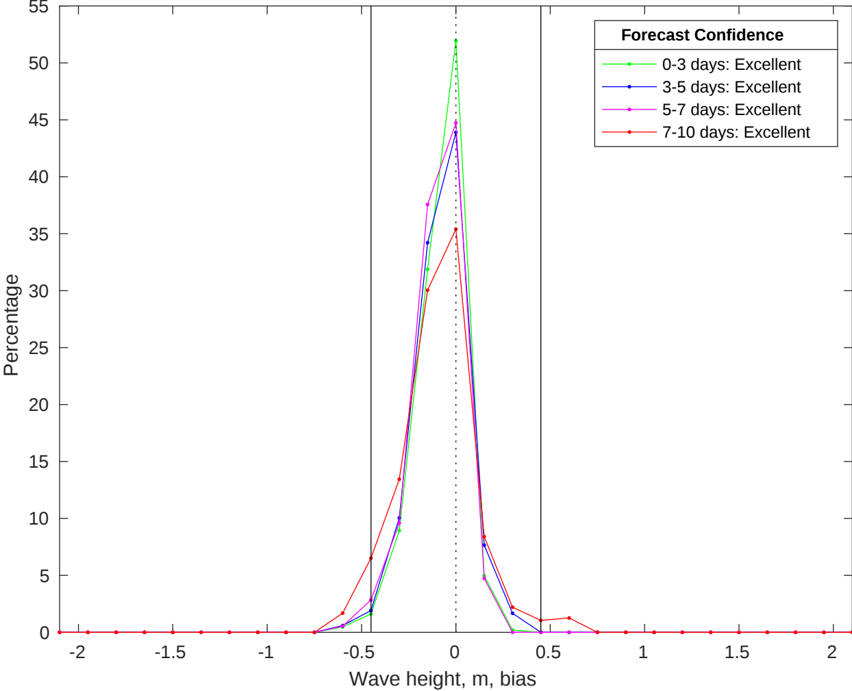
NDBC 42040 vs CMEMS Waves Bias Histogram: 29-Jun-2025
