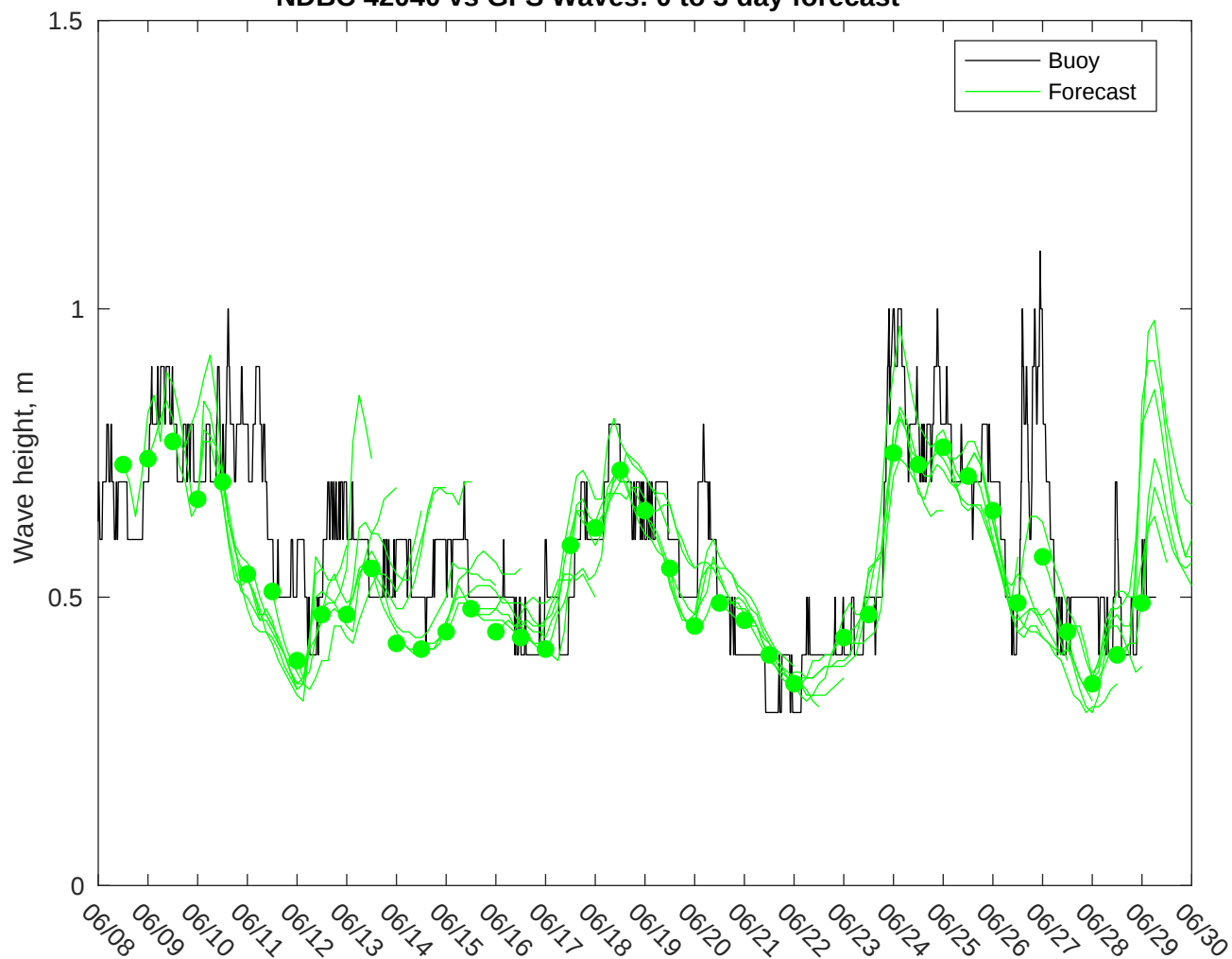
NDBC 42040 vs GFS Waves: 0 to 3 day forecast
