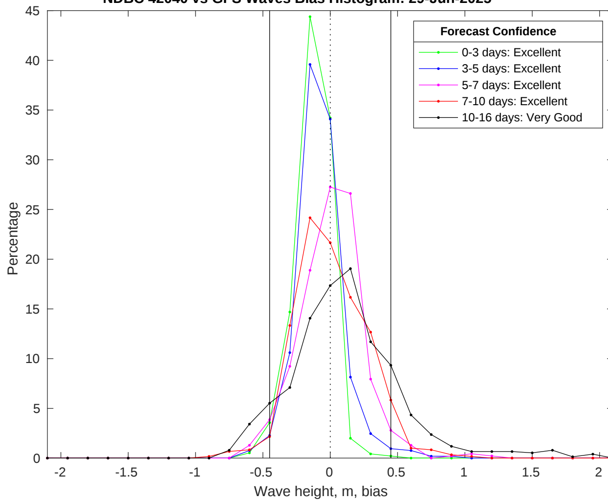
NDBC 42040 vs GFS Waves Bias Histogram: 29-Jun-2025
