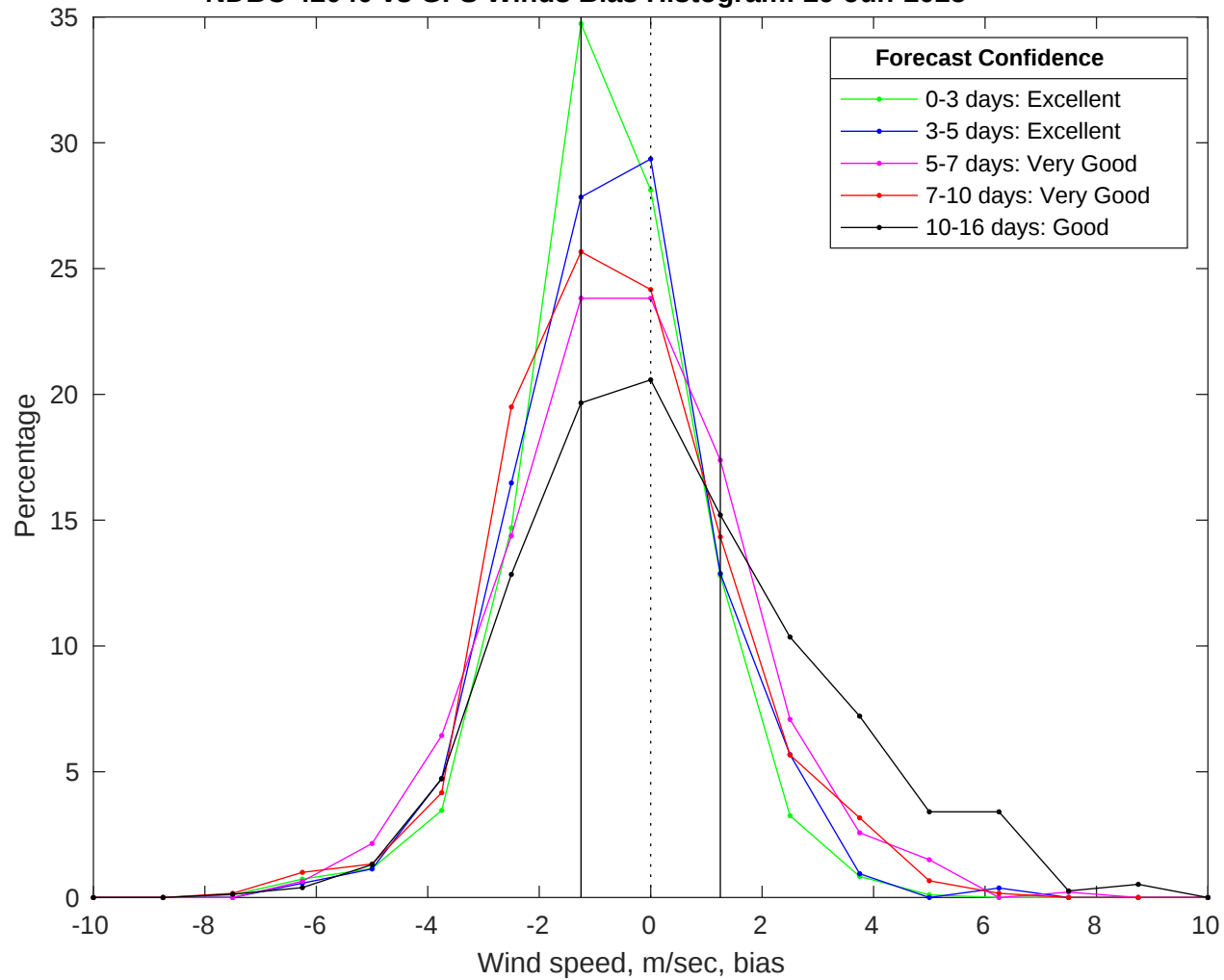
NDBC 42040 vs GFS Winds Bias Histogram: 29-Jun-2025
