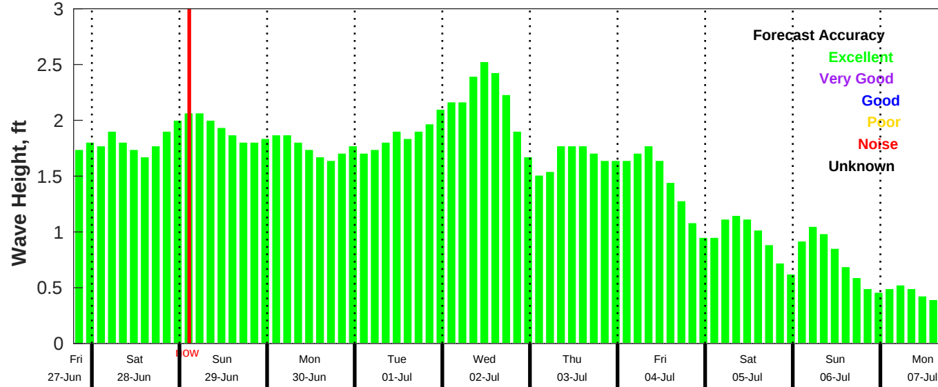
CMEMS Wave Forecast for NDBC 42040 from 27-Jun-2025 19:00:00 to 07-Jul-2025 19:00:00
