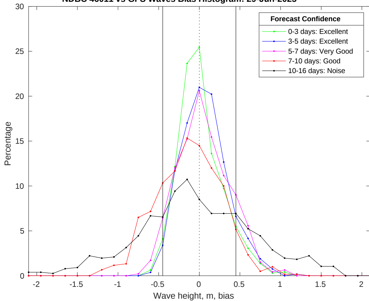
NDBC 46011 vs GFS Waves Bias Histogram: 29-Jun-2025
