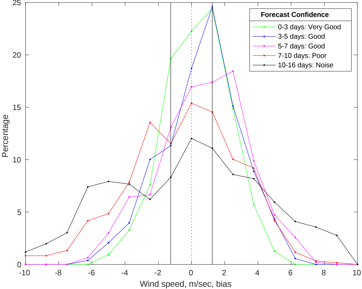
NDBC 46011 vs GFS Winds Bias Histogram: 29-Jun-2025
