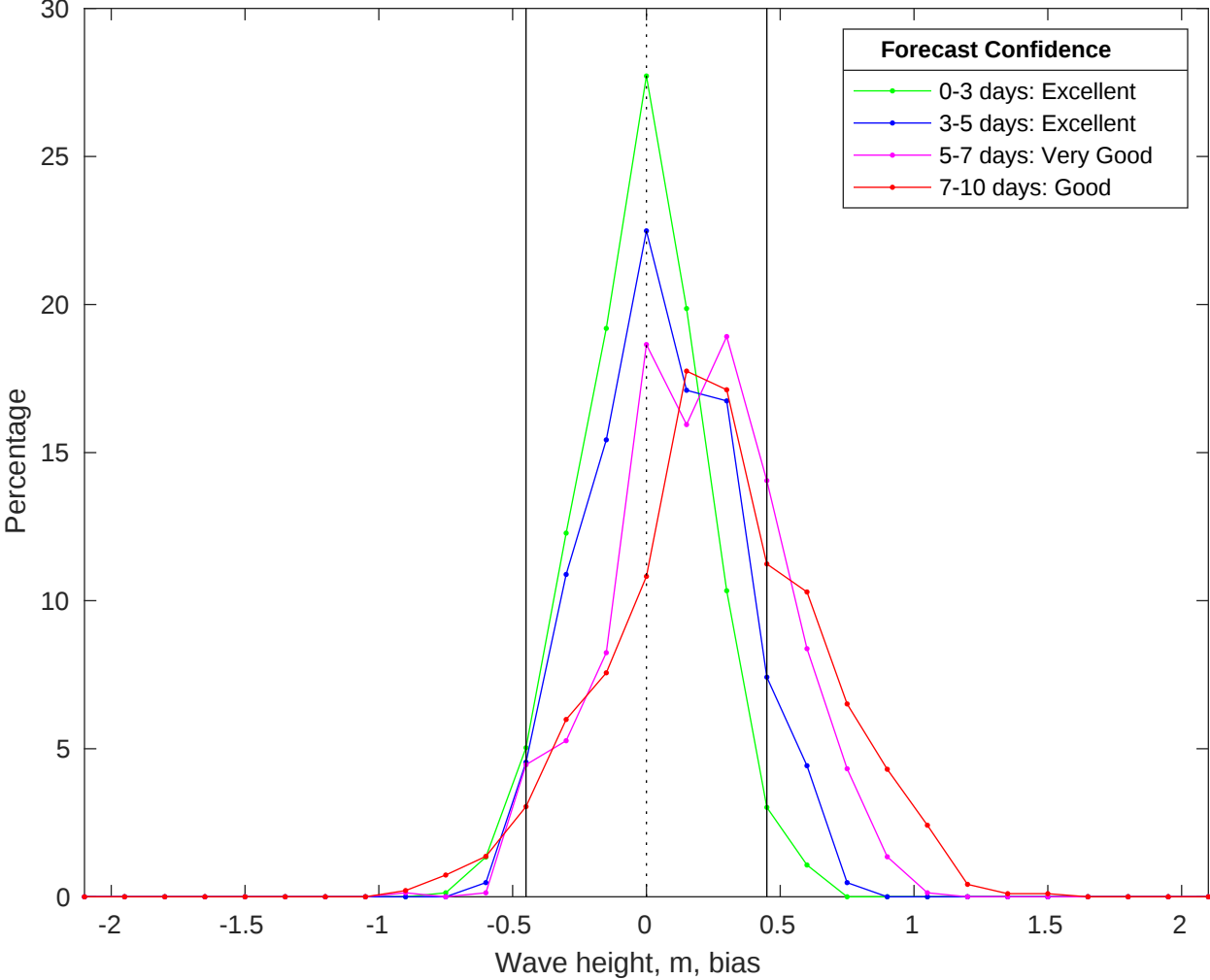
NDBC 46028 vs CMEMS Waves Bias Histogram: 29-Jun-2025
