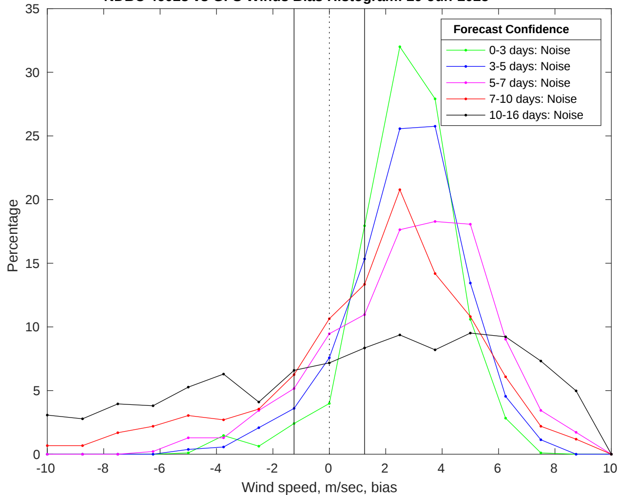
NDBC 46028 vs GFS Winds Bias Histogram: 29-Jun-2025
