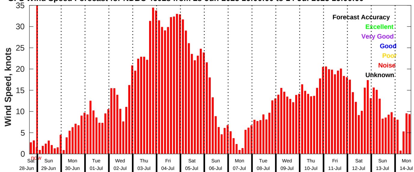
GFS Wind Speed Forecast for NDBC 46028 from 28-Jun-2025 16:00:00 to 14-Jul-2025 16:00:00
