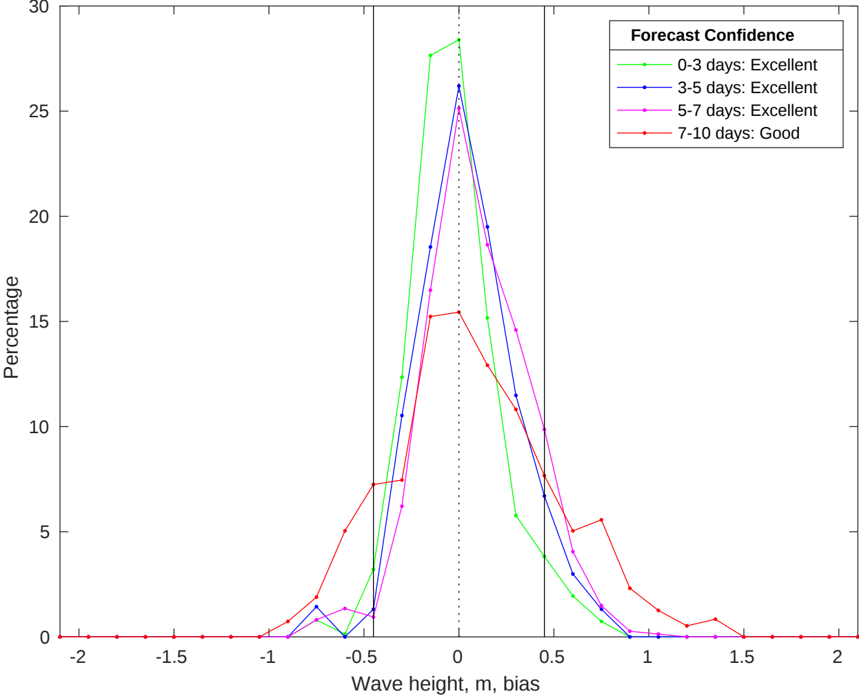
NDBC 46054 vs CMEMS Waves Bias Histogram: 29-Jun-2025
