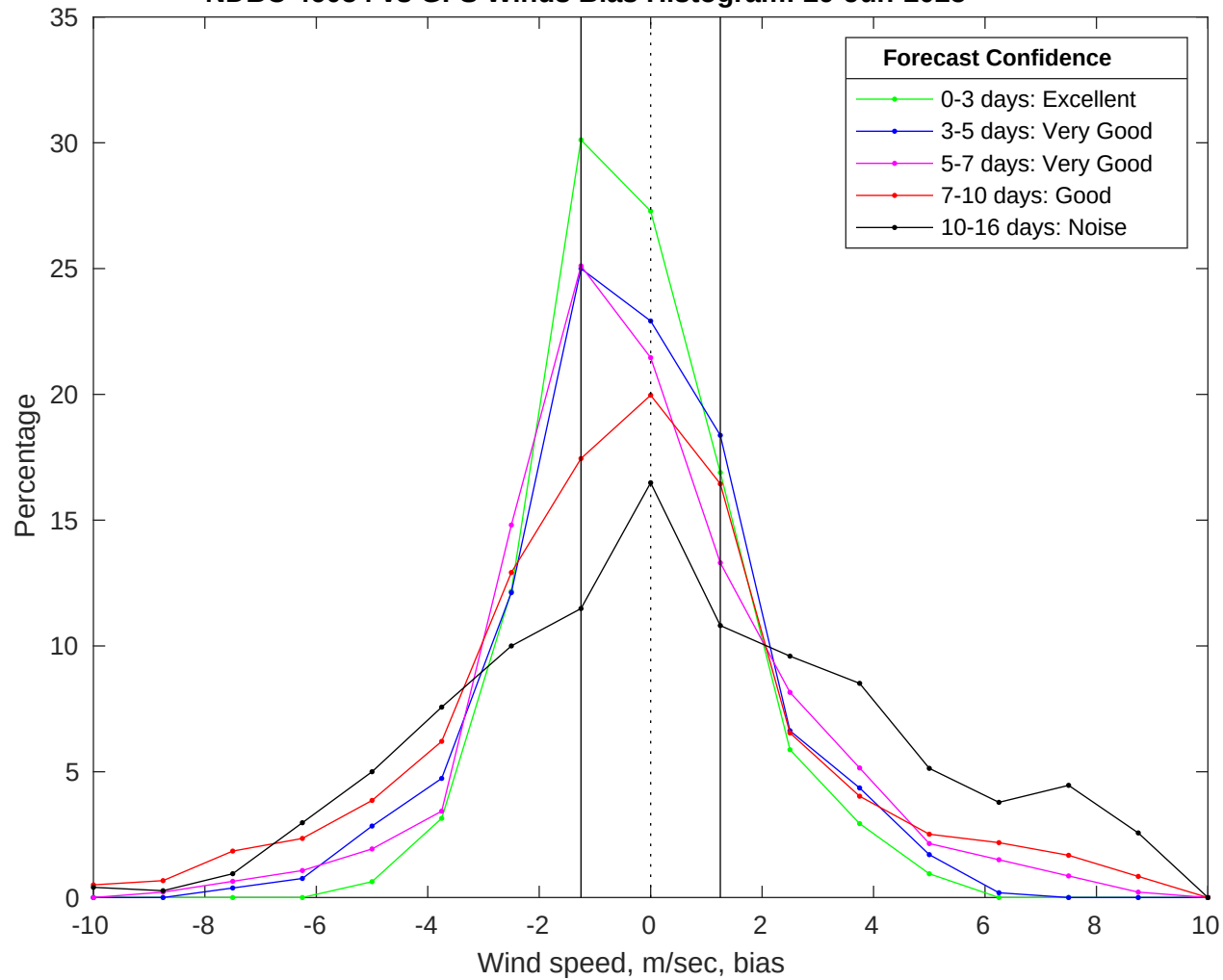
NDBC 46054 vs GFS Winds Bias Histogram: 29-Jun-2025
