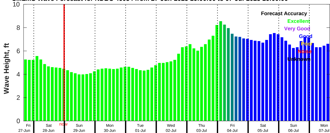
CMEMS Wave Forecast for NDBC 46054 from 27-Jun-2025 16:00:00 to 07-Jul-2025 16:00:00
