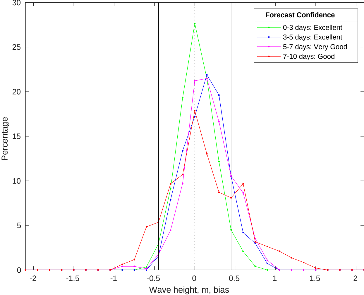
NDBC 46069 vs CMEMS Waves Bias Histogram: 29-Jun-2025
