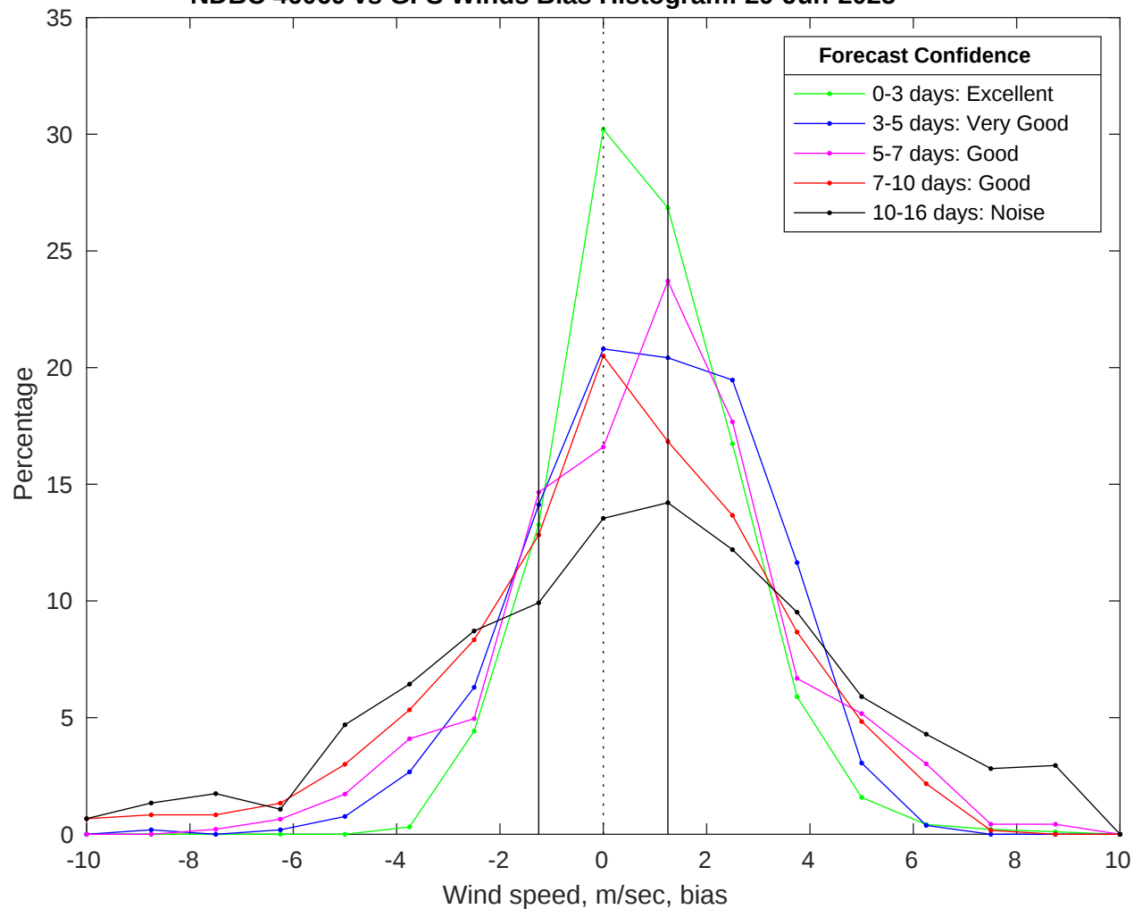
NDBC 46069 vs GFS Winds Bias Histogram: 29-Jun-2025
